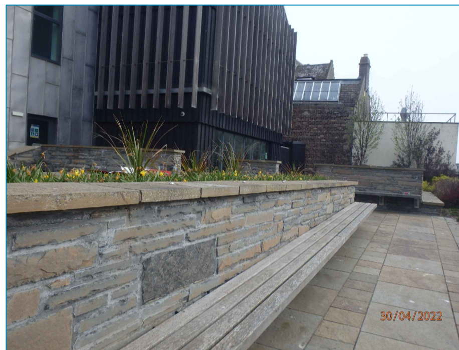
Caithness flagstone planters with built in bench seating.
