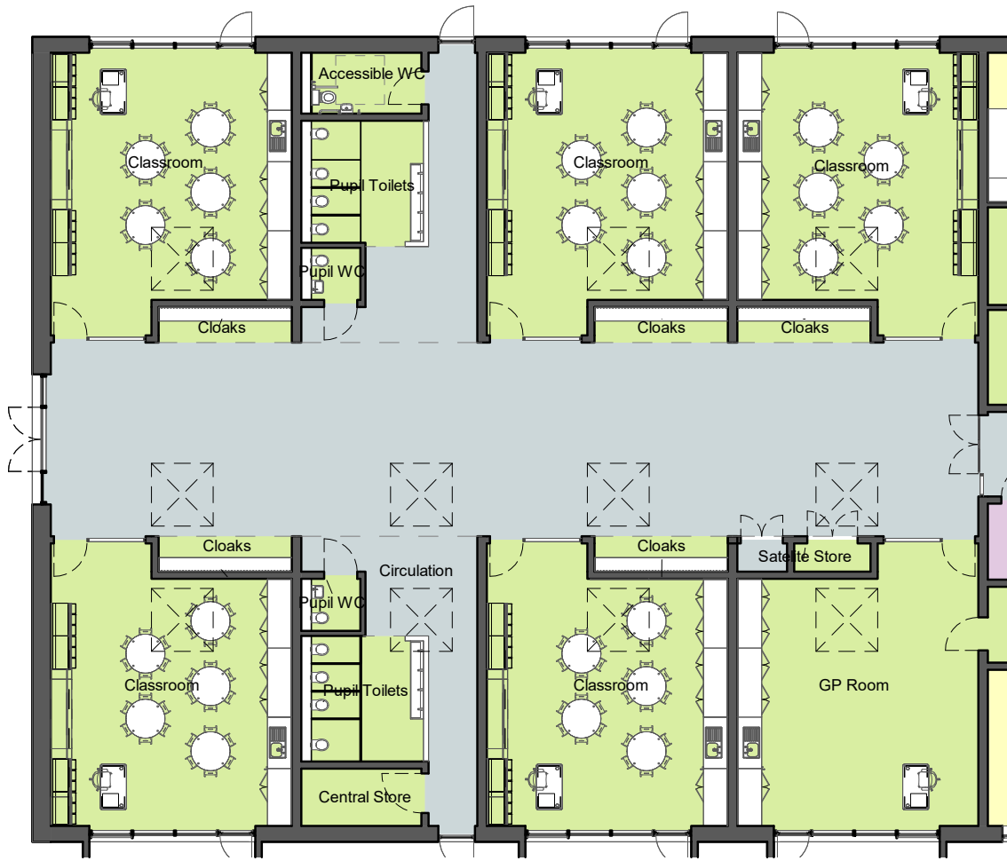
Classroom Block Plan 1:200
