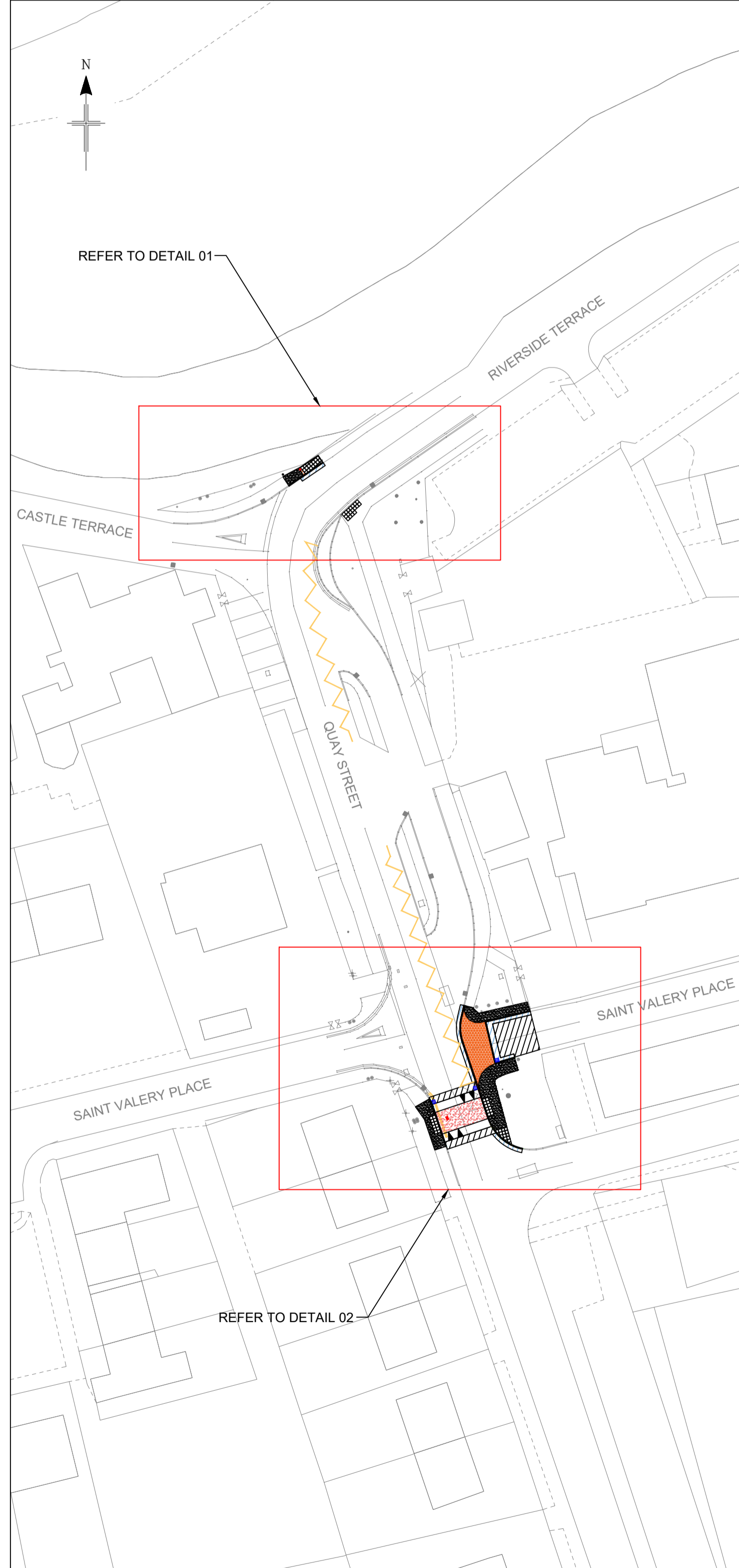
GENERAL LAYOUT SCALE 1:500
