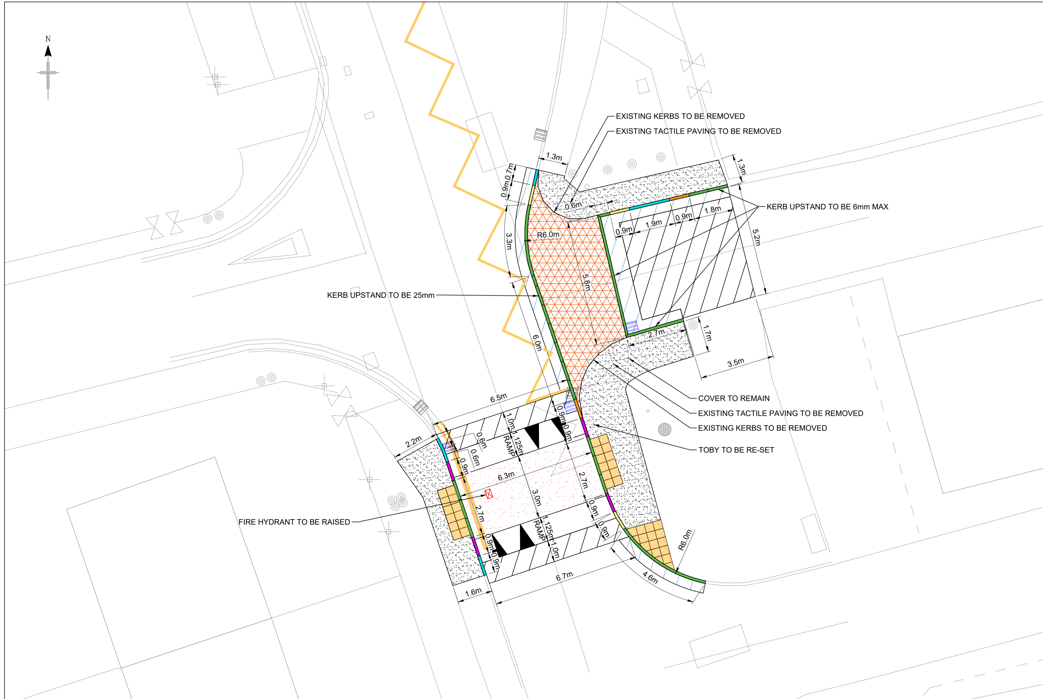
DETAIL 02 SCALE 1:100
