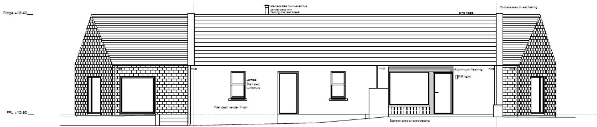
South Elevation
