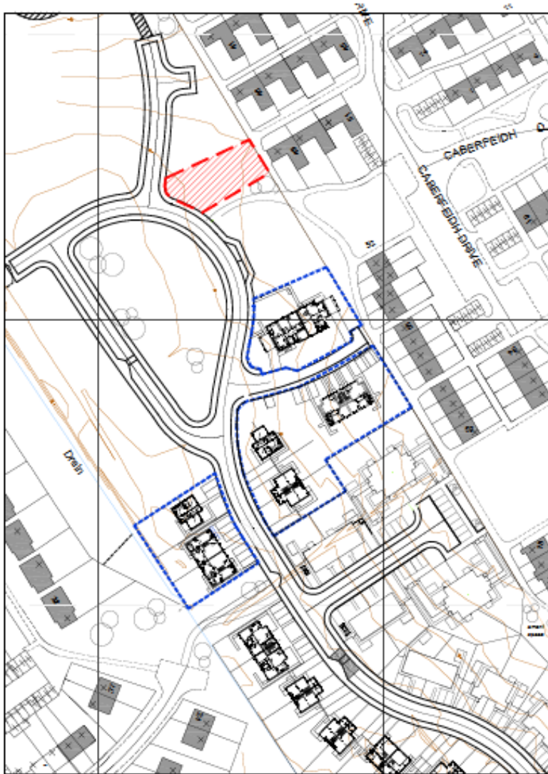
LOCATION PLAN 1:1000
