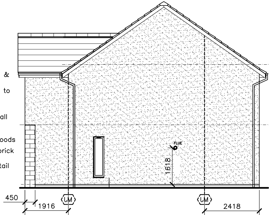
RIGHT GABLE ELEVATION
