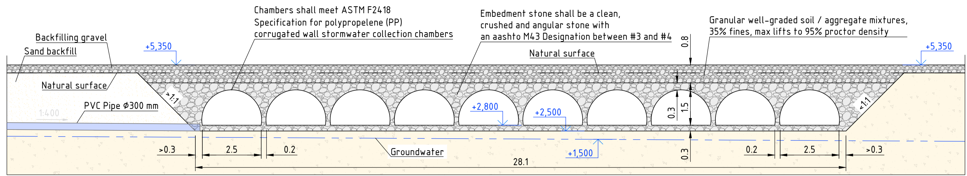
Section 9-9 1:100
