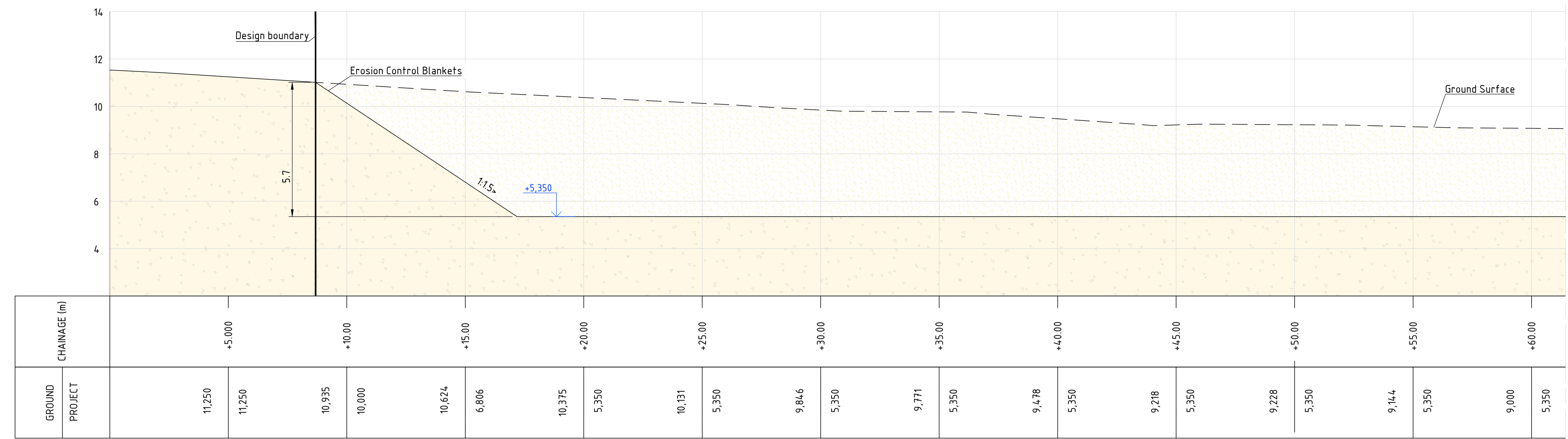
Section 4-4 1:100
