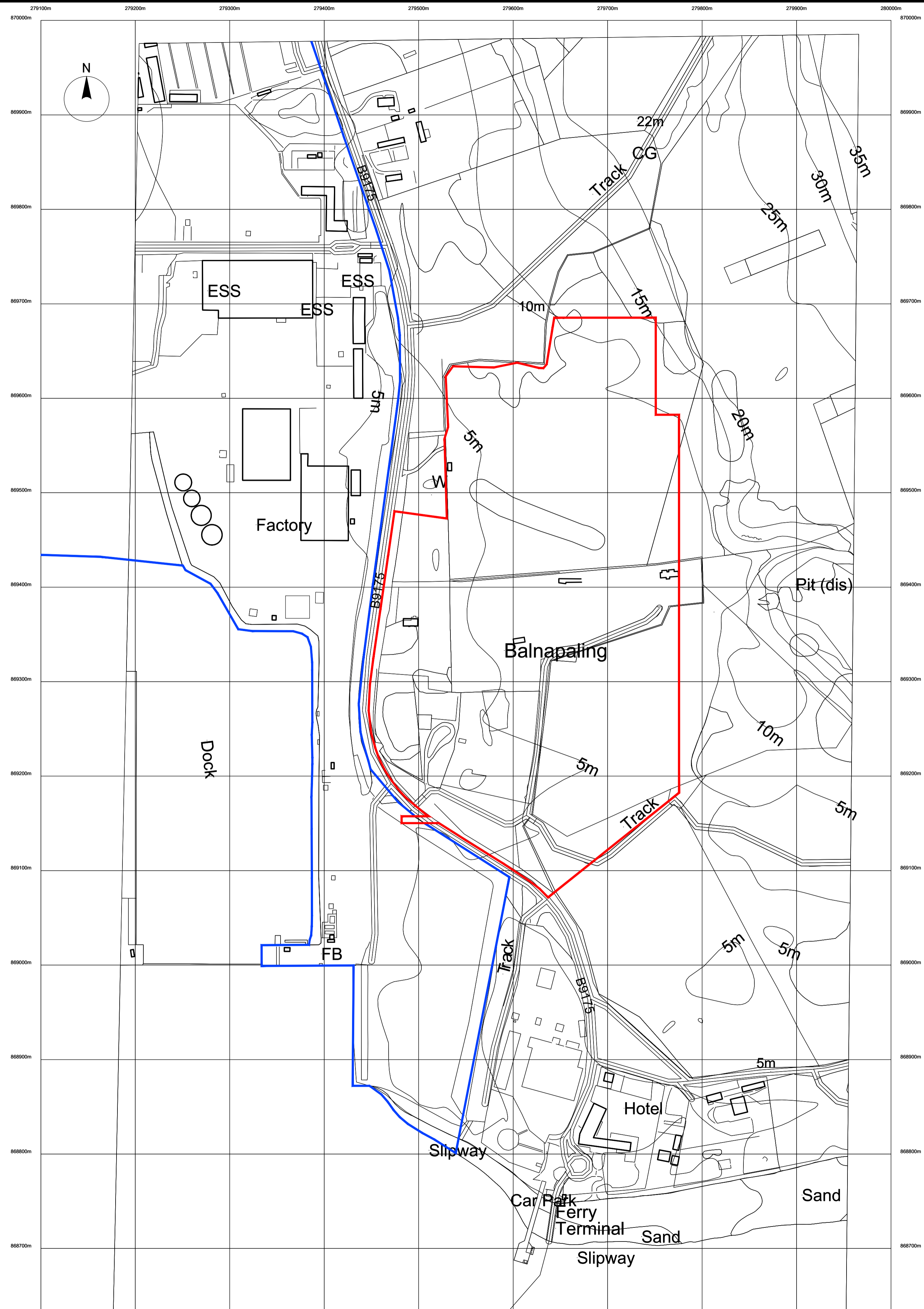
Site Location Map 1:2500 1:2500 scale bar 0 25m 100m
