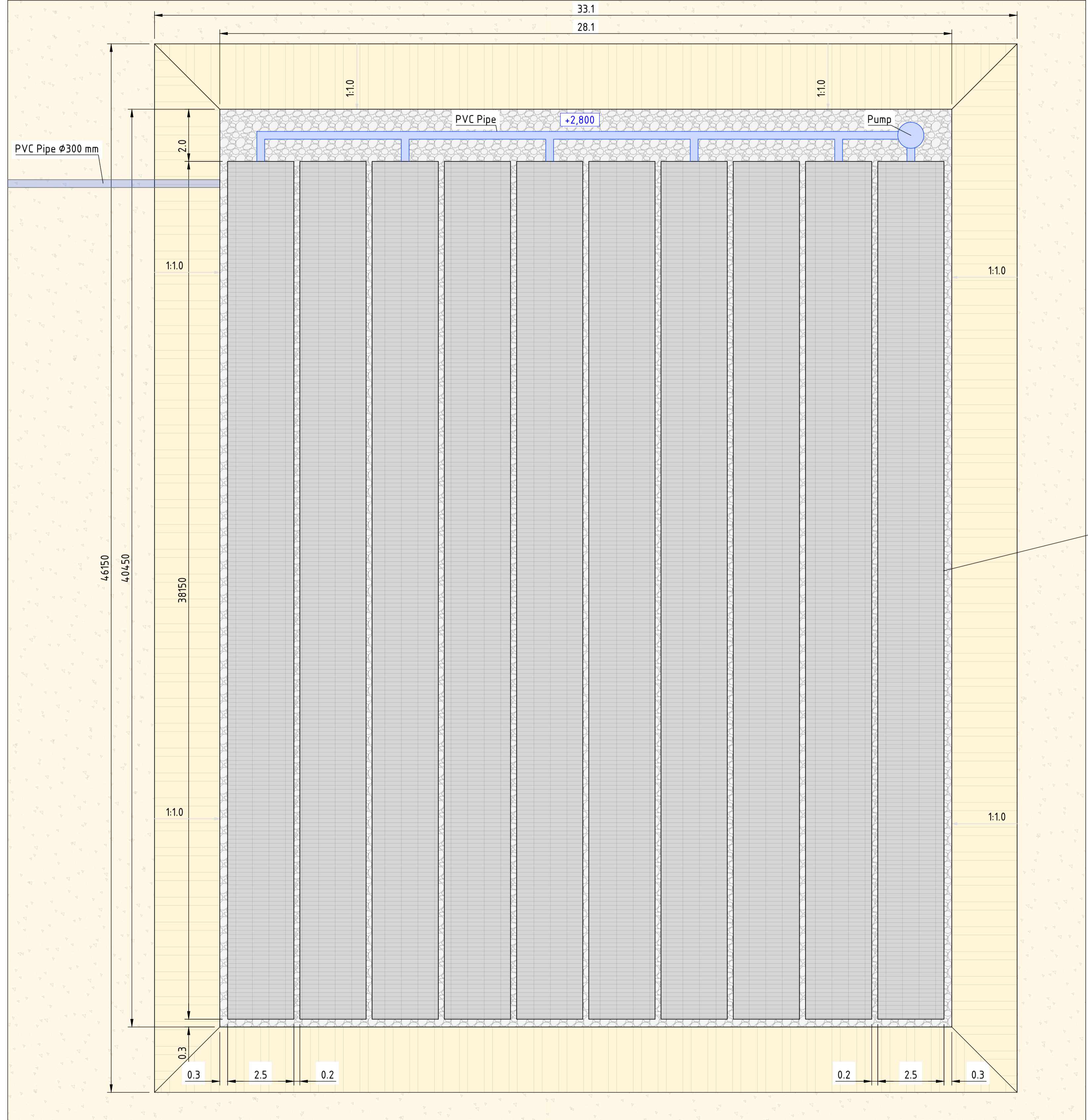
Plan (Shown without backfill) 1:100
