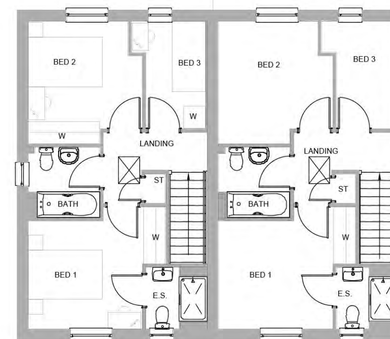
FIRST FLOOR 1:100
