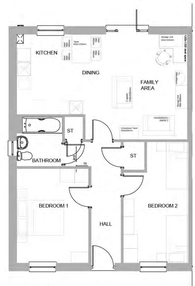
GROUND FLOOR 1:100
