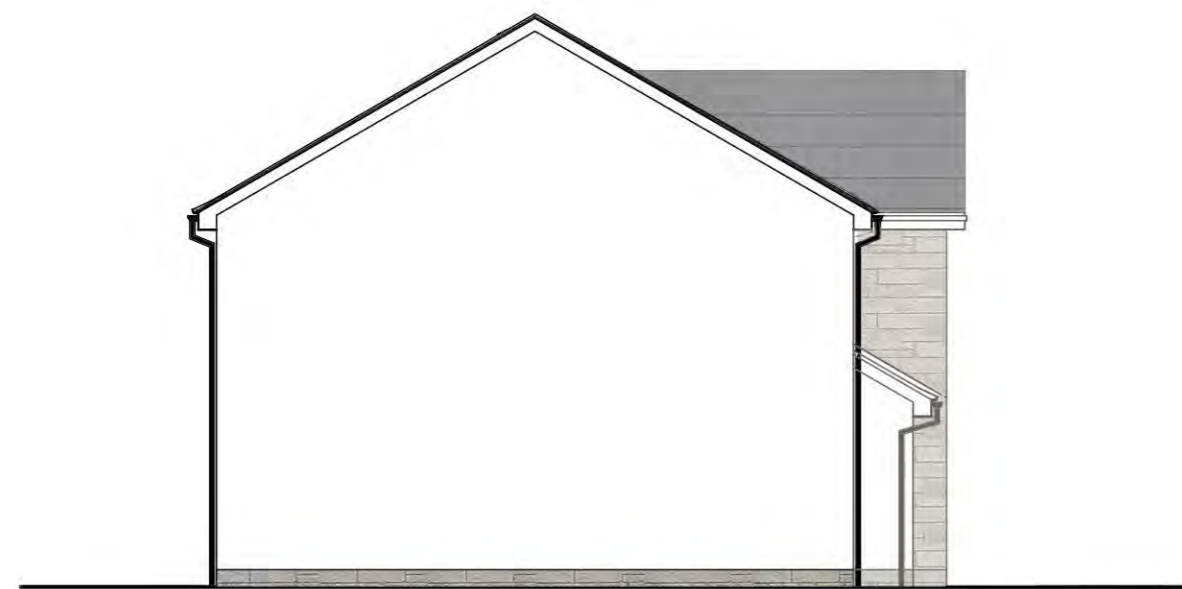
SIDE ELEVATION 1:100
