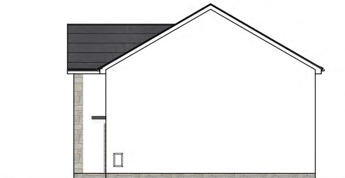
SIDE ELEVATION 1:100
