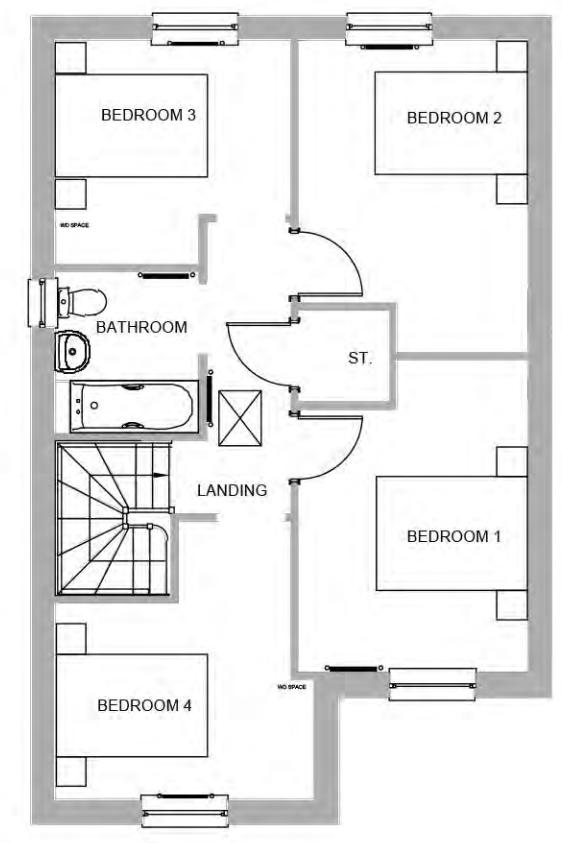
FIRST FLOOR 1:100
