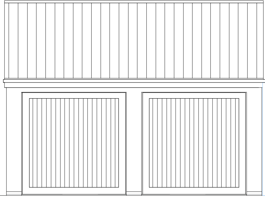
FRONT ELEVATION
