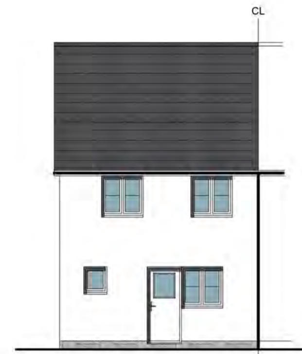
REAR ELEVATION
