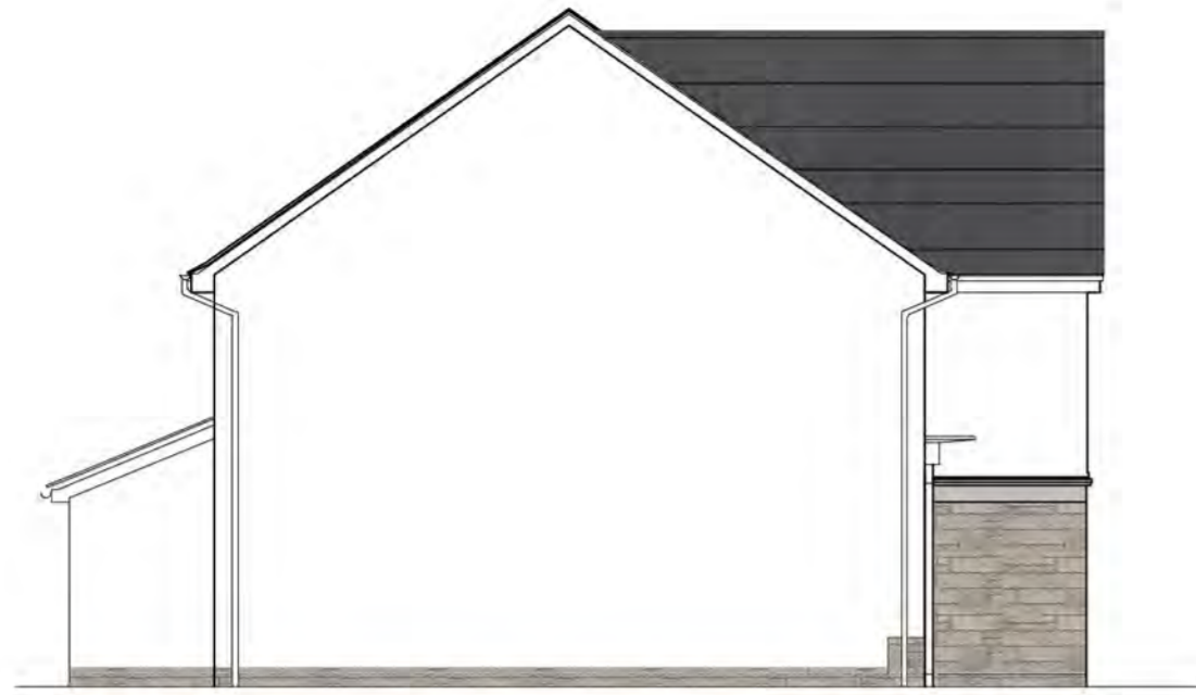
SIDE ELEVATION 1:100
