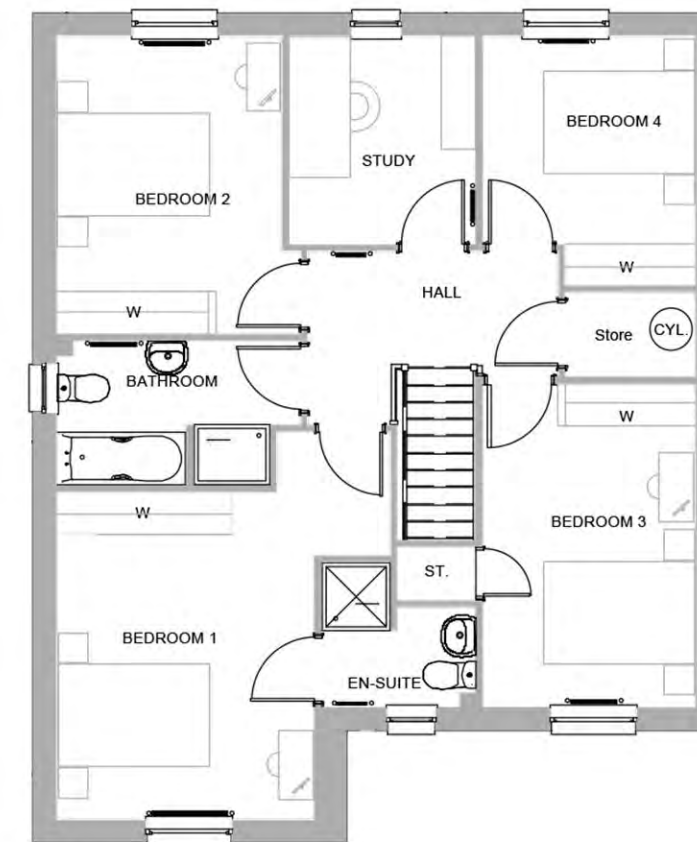
FIRST FLOOR 1:100
