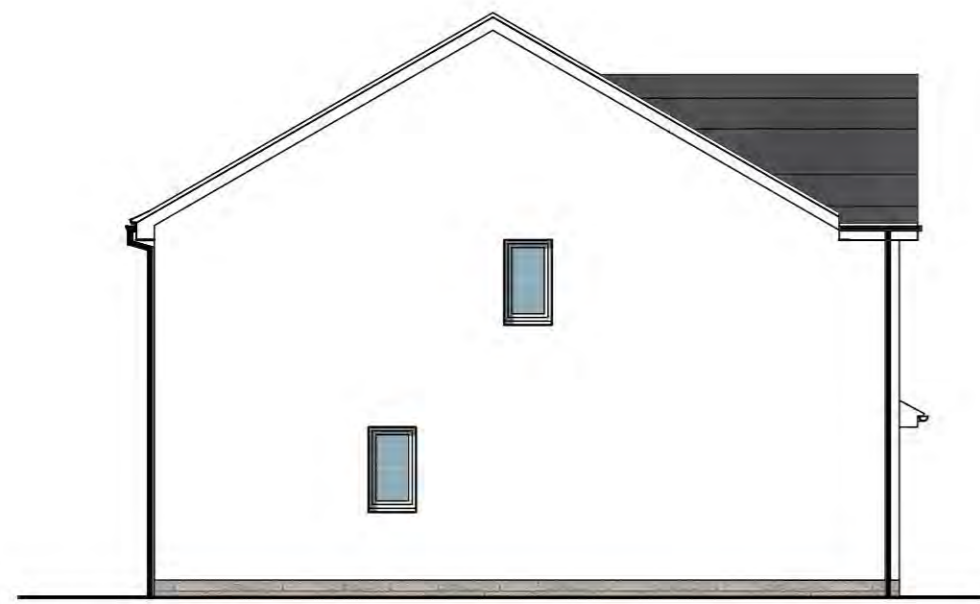
SIDE ELEVATION 1:100
