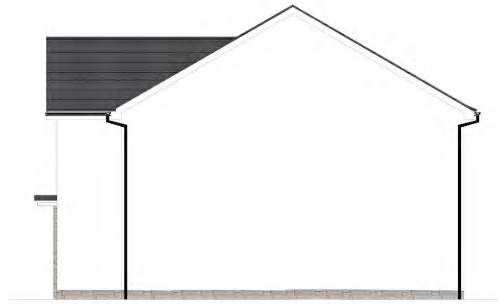
SIDE ELEVATION 1:100
