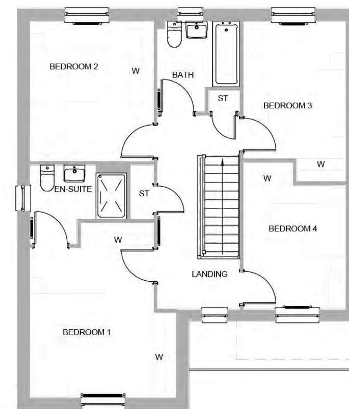
FIRST FLOOR 1:100
