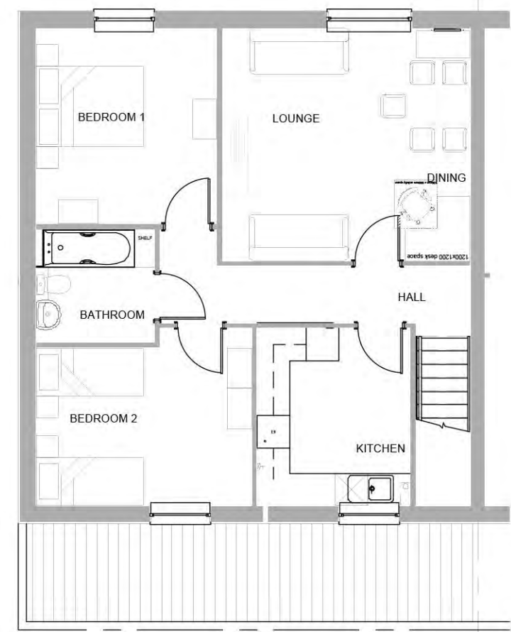
FIRST FLOOR 1:100
