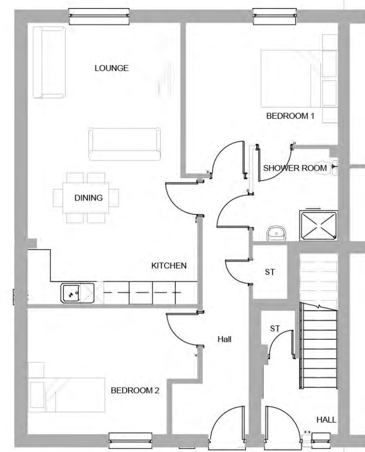
GROUND FLOOR 1:100
